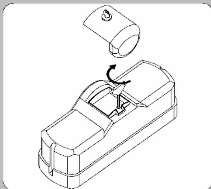
Fit the Allen key and turn it clockwise. Do not force the Allen key but move the leaf door at the same time to make sure it has been released.
